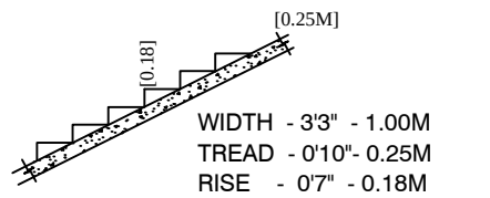
STAIRCASE DETAILS
