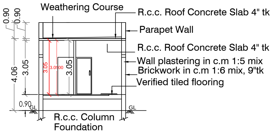
SECTION NN
