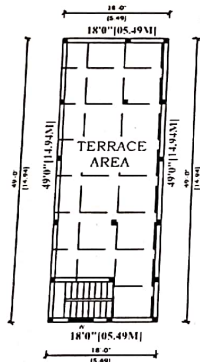
TERRACE FLOOR
