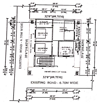
PRO.GROUND FLOOR
