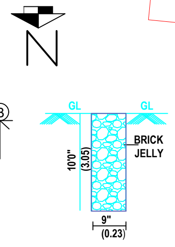
PERCULATION PIT
