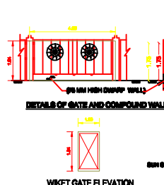
WIKET GATE ELEVATION
