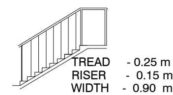
STAIRCASE DETAILS
