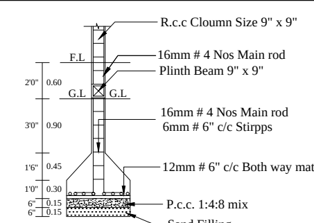
COLUMN DETIAL
