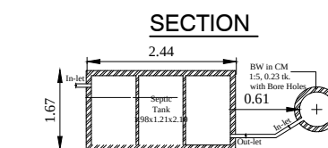
PLAN - SEPTIC TANK & SOAK PIT
