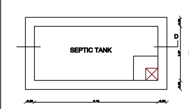
PLAN OF SEPTIC TANK SCALE 1"=2'0"
