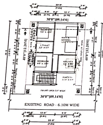
PRO. GROUND FLOOR
