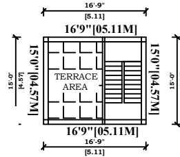
TERRACE FLOOR
