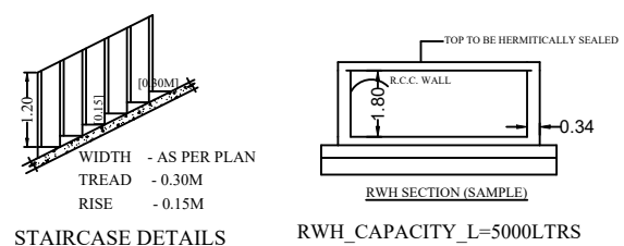
STAIRCASE DETAILS
