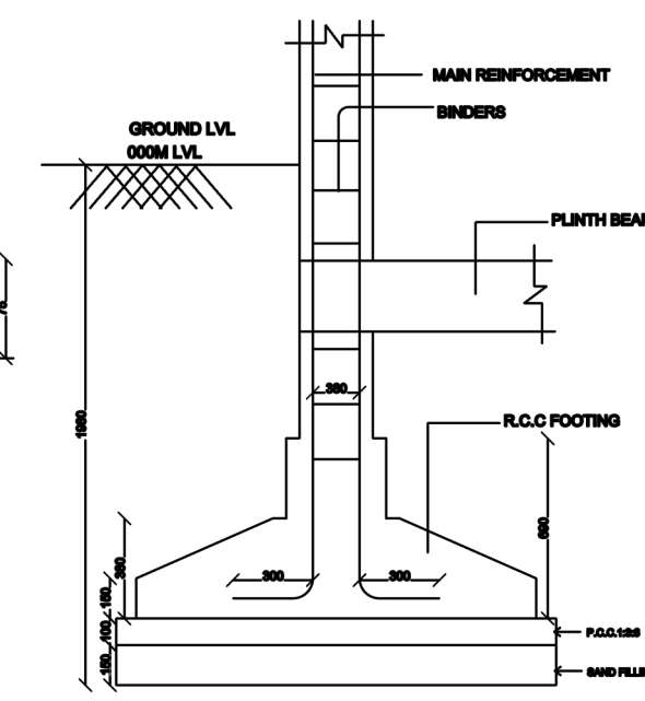
TYPICAL SECTION OF R.C.C COLUMN FOUNDATION SCALE: 1"=2'0"
