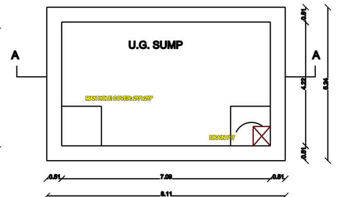
SUMP DETAIL
