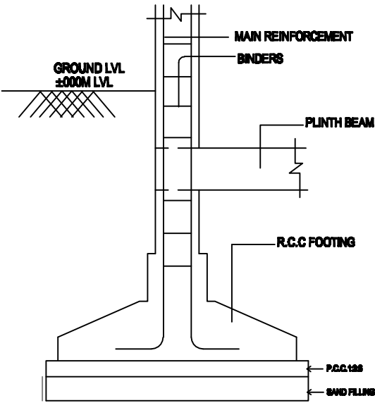
TYPICAL SECTION OF R.C.C COLUMN FOUNDATION SCALE: 1"=8"
