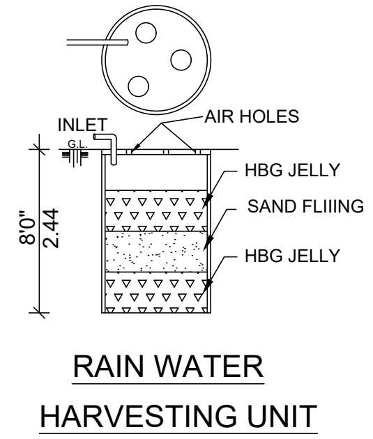
RWH SECTION(SAMPLE)
