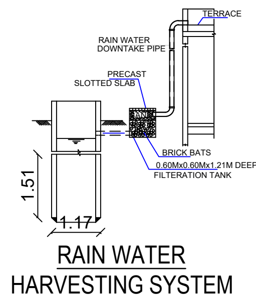
RWH SECTION(SAMPLE)
