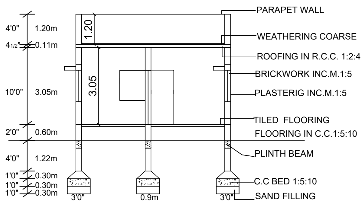
SECTION ON"AA"
