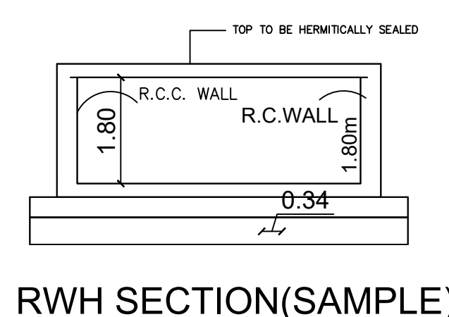
RWH SECTION(SAMPLE)
