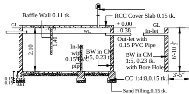
SECTION PLAN - SEPTIC TANK & SOAK PIT NOT TO SCALE
