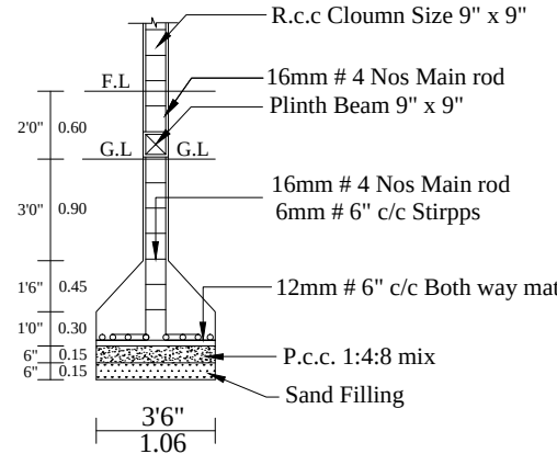
COLUMN DETIAL
