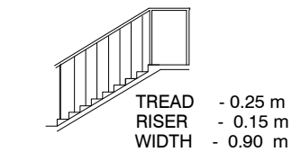
STAIRCASE DETAILS
