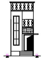
FRONT ELEVATION
