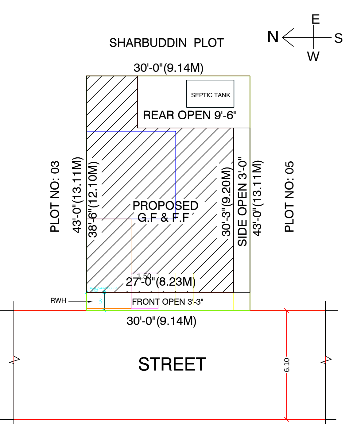
SITE PLAN
