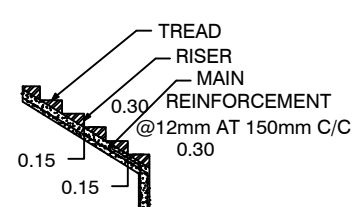
STAIRCASE DETAILS
