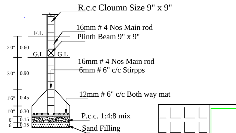
COLUMN DETAIL
