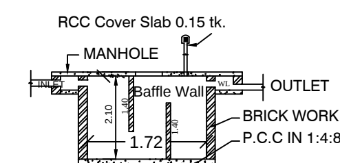
SECTION - SEPTIC TANK
