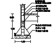
COLUMN DETAILS
