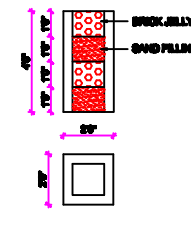
PERCOLATION PIT
