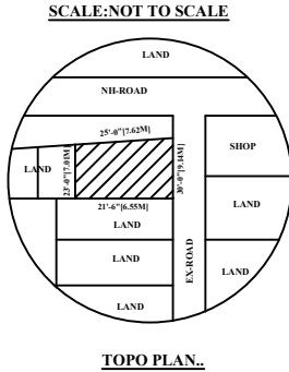
TOPO PLAN..
