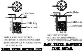
RAIN WATER HARVESTING UNIT
