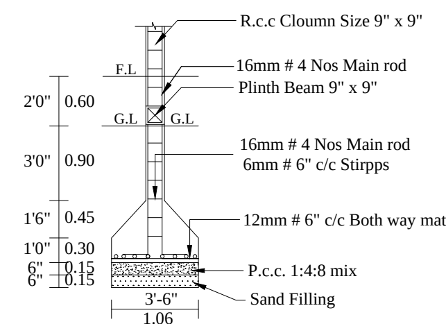
COLUMN DETIAL
