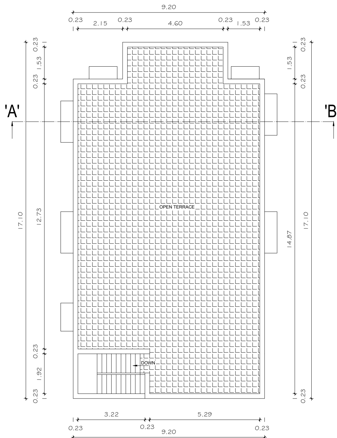
PRO. TERRACE FLOOR PLAN.
