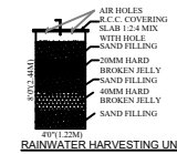
RAIN WATER HARVESTING UNIT SIZE: 4'0" X 4'0" X 10'0" - 3 NOS NOTE: 1. RAIN PIPE AND NECESSARY SPECIALS
