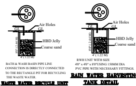
RAIN WATER HARVESTING TANK DETAIL SCALE: 1:50
