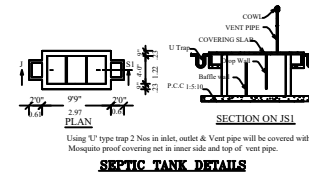
SEPTIC TANK DETAILS SCALE: 6'0" X 3'0" X 6'0"
