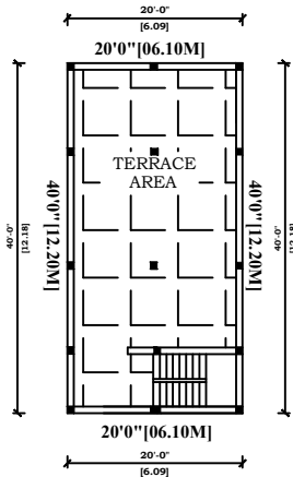
TERRACE FLOOR
