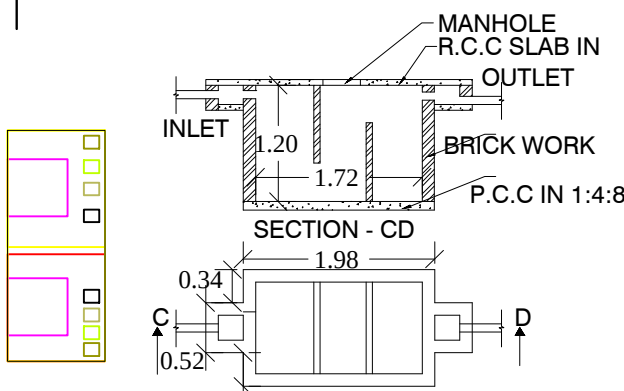
PLAN OF SEPTICK TANK
