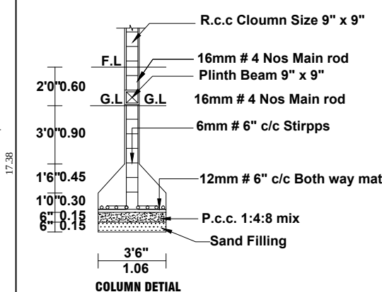
COLUMN DETAIL
