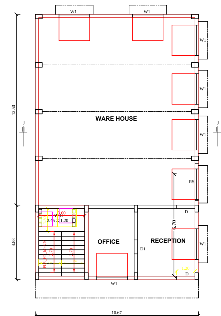
G F PLAN
