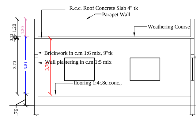
SECTION ON JJ
