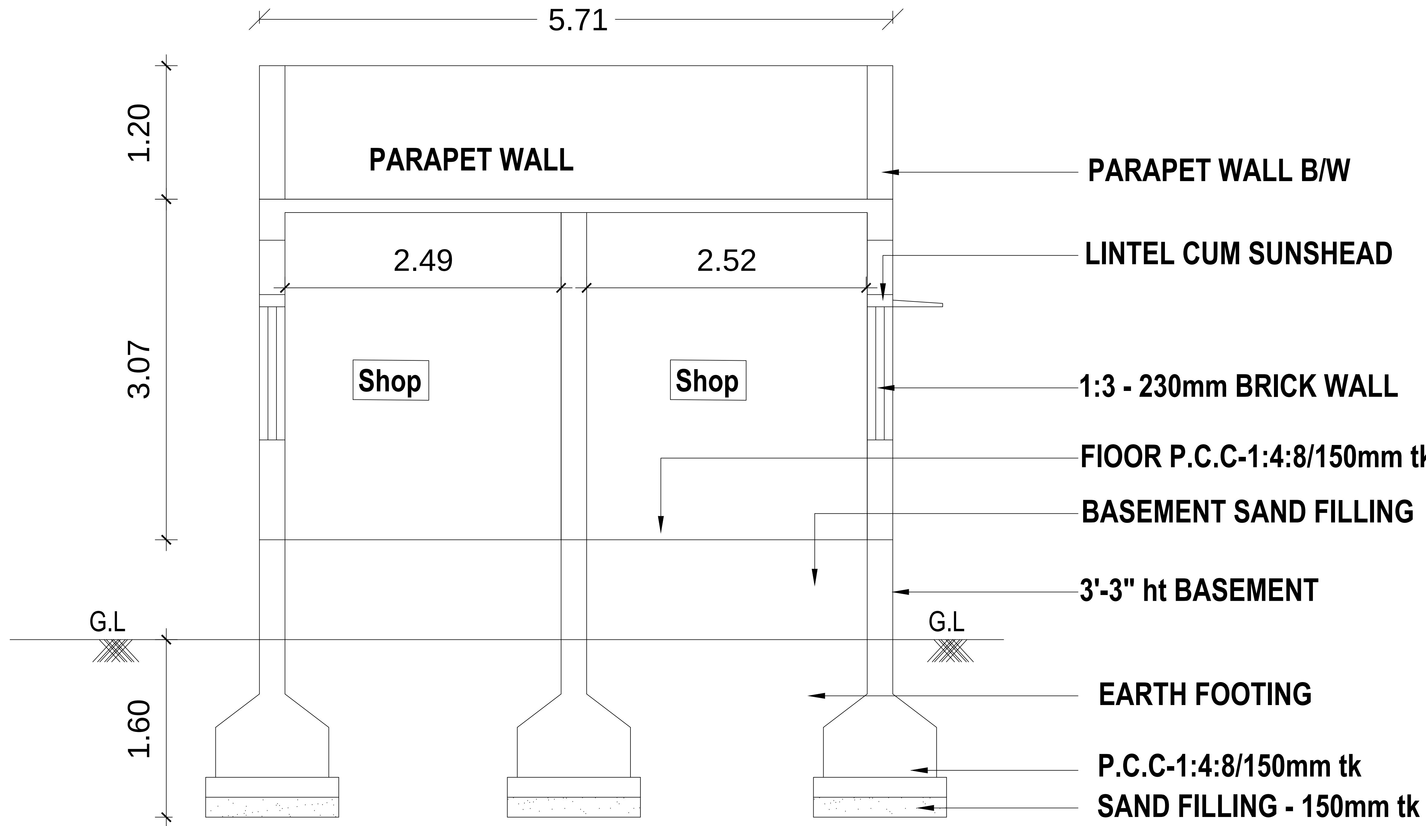
SECTION -A-A'
