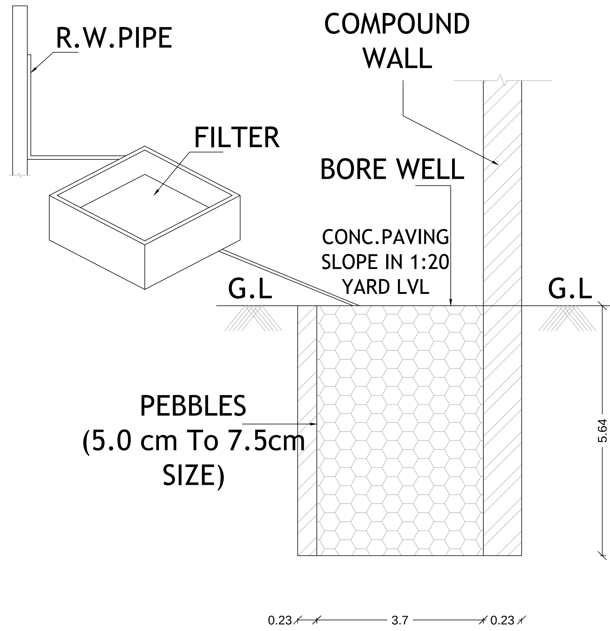
RAIN WATER TRENCH
