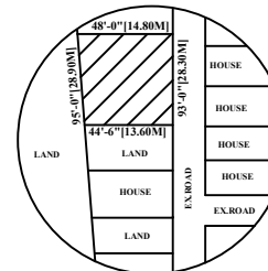
TOPO PLAN..
