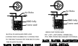
RAIN WATER HARVESTING TANK DETAIL
