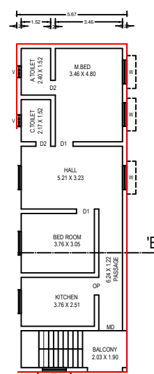
RO. FIRST FLOOR PLAN.
