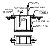
SEPTIC TANK DETAILS
