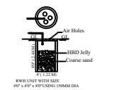
RAIN WATER HARVESTING UNIT
