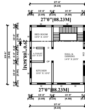
PRO.FIRST FLOOR PLAN
