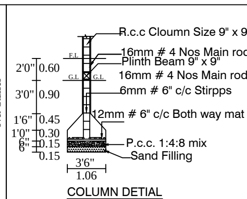
COLUMN DETAIL
