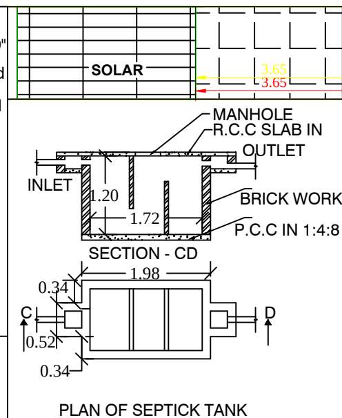
PLAN OF SEPTICK TANK
