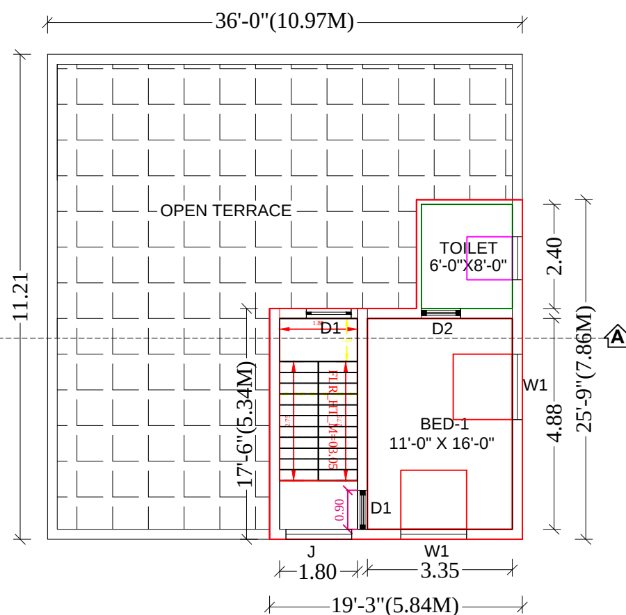
FIRST FLOOR & HEAD ROOM PLAN
