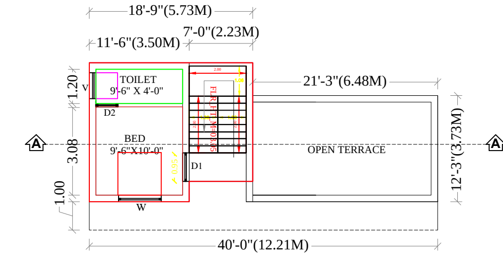
PRO. ADDITIONAL FIRST FLOOR PLAN
