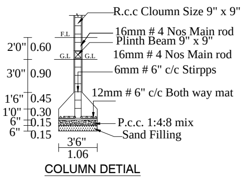
COLUMN DETIAL
