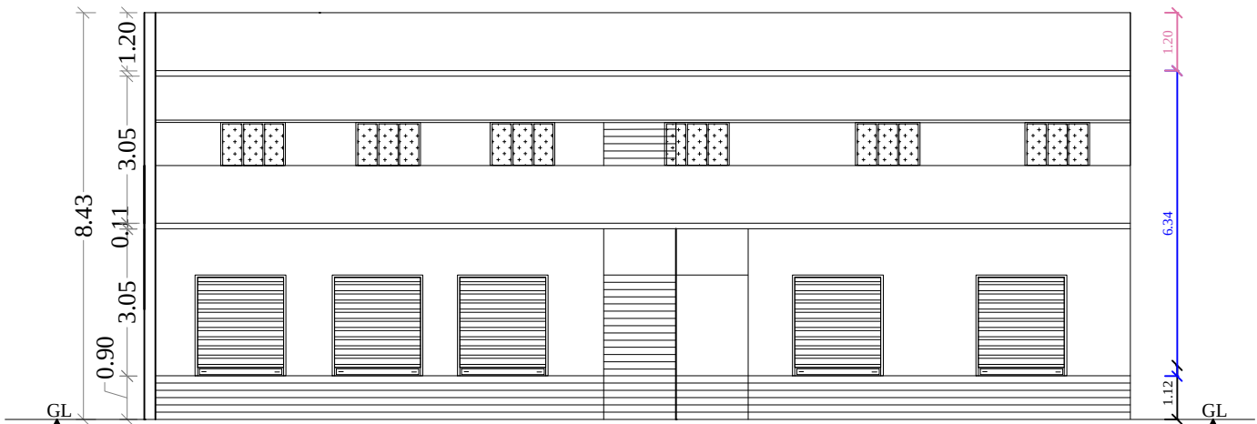
FRONT ELEVATION
