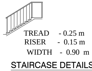
STAIRCASE DETAILS
