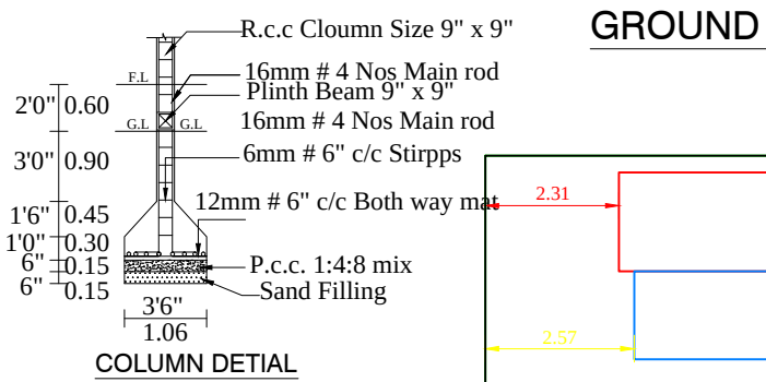
COLUMN DETIAL
