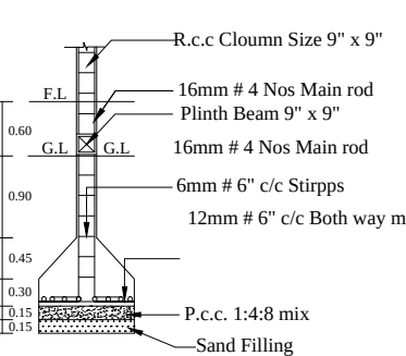
COLUMN DETIAL NOT TO SCALE
