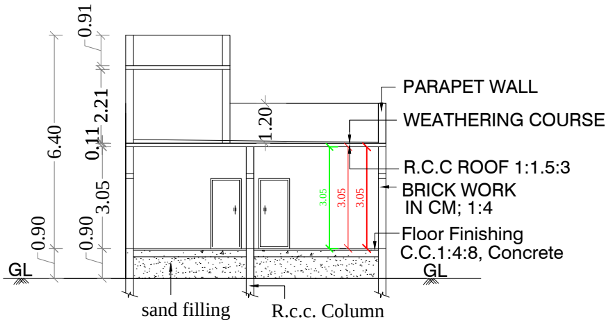
SECTION ON NN
