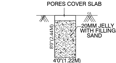
RAIN WATER HARVESTING UNIT
