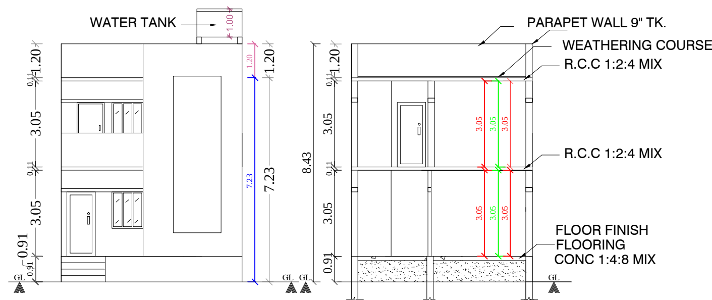
FRONT ELEVATION
