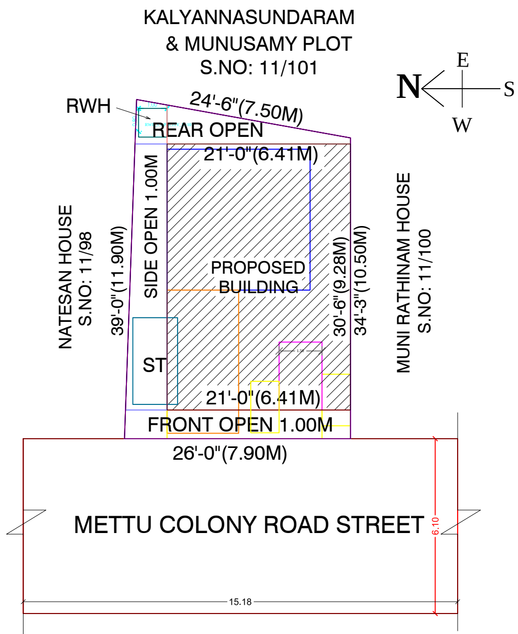
SITE PLAN (SCALE: 1CM : 1M)
