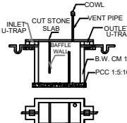
SEPTIC TANK DETAILS SIZE: 6'0" x 3'0" x 6'0"
