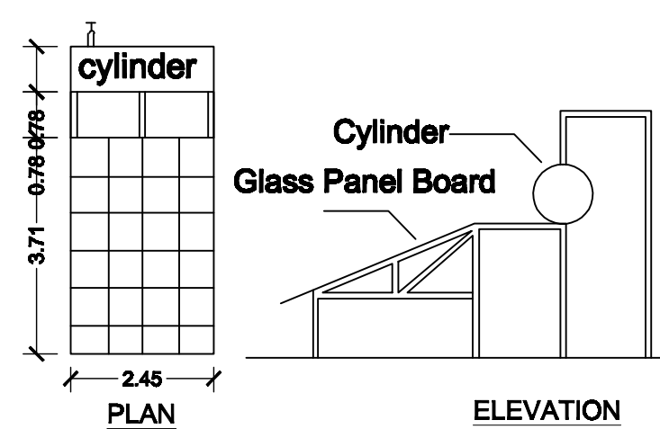
SOLAR ENERGY SYSTEM
