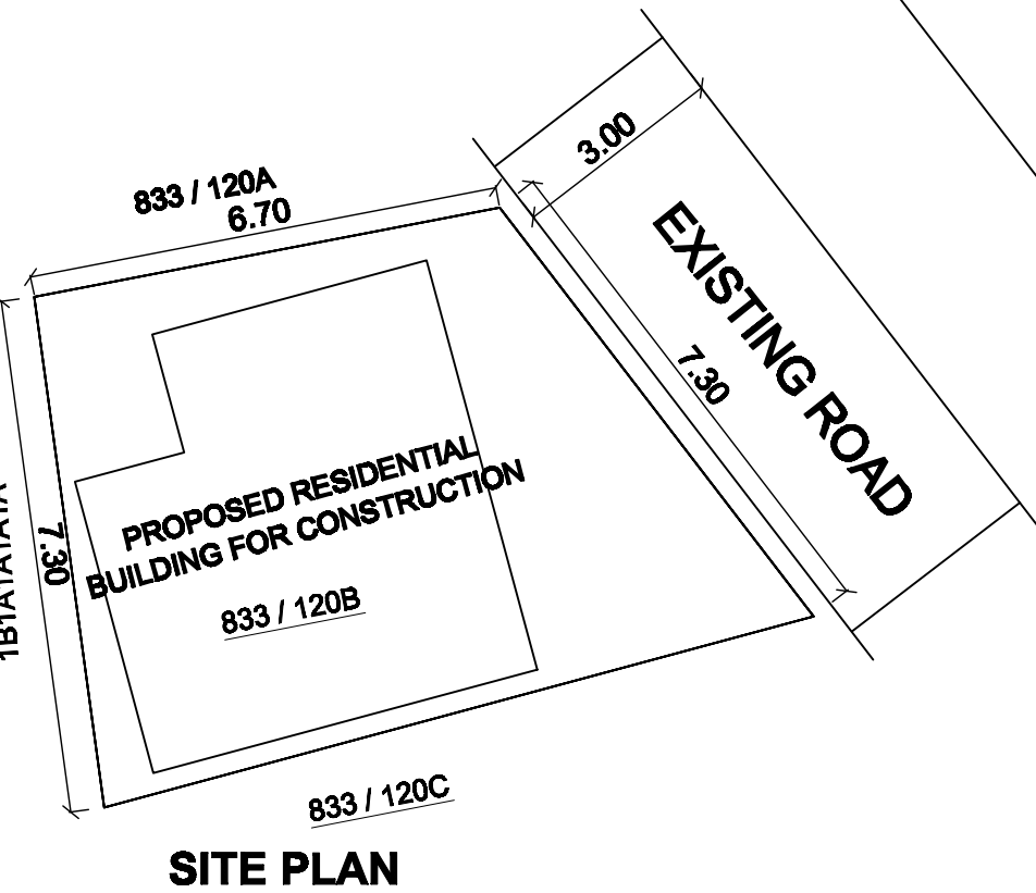
SITE PLAN
