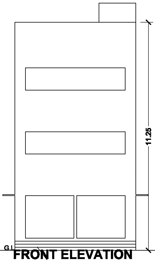
FRONT ELEVATION
