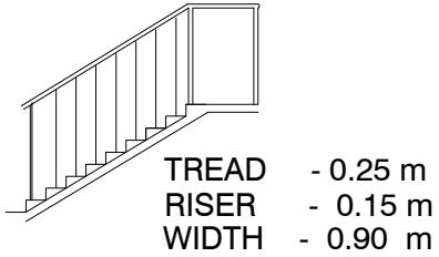
STAIRCASE DETAILS
