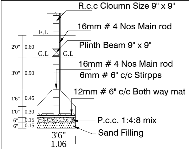
COLUMN DETIAL
