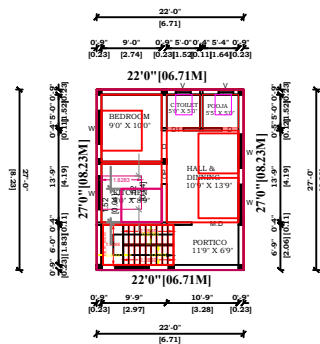
PRO. FIRST FLOOR PLAN
