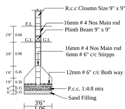
COLUMN DETAIL
