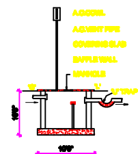
SEPTIC TANK DETAILS
