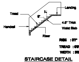
STAIRCASE DETAIL
