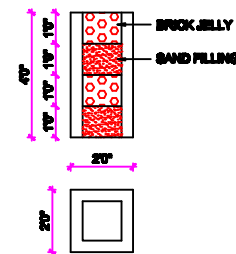
PERCOLATION PIT
