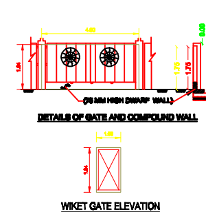
WIKET GATE ELEVATION
