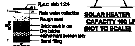
RAIN WATER HARVEST UNIT
