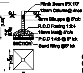
FOUNDATION DETAIL
