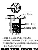
WASTE WATER RECYCLING UNIT
