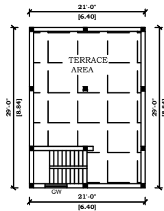
TERRACE FLOOR
