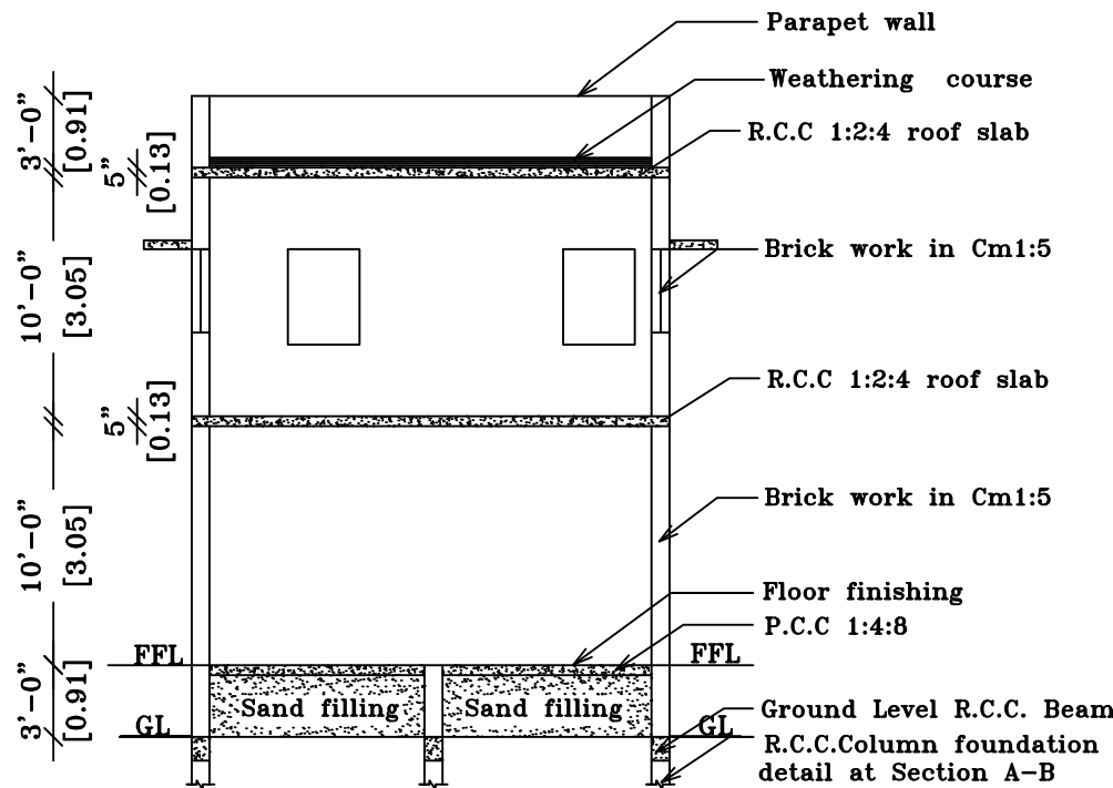
SECTION ON 'SA'
