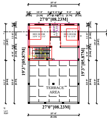
PRO.FIRST FLOOR...
