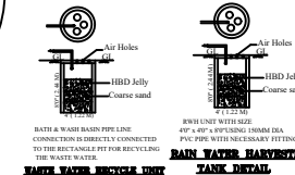
WATER HARVESTING UNIT
