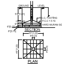
FOUNDATION DETAILS
