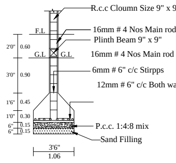
COLUMN DETAIL
