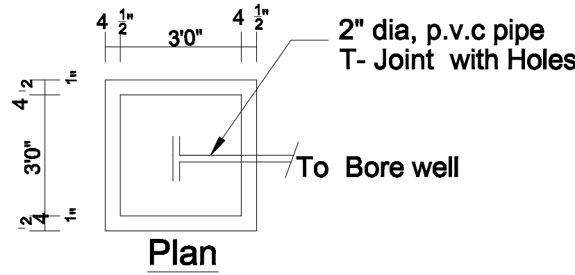
RAINWATER HARVESTING TANK SCALE 1:50
