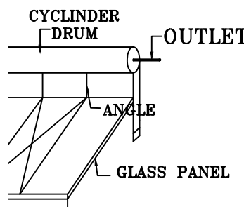
ENERGY SCALE
