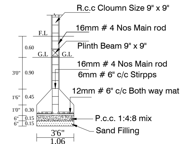
COLUMN DETIAL
